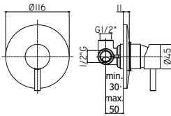
LIG 010-011CR Miscelatore incasso doccia / Piastra Ø116 e 110 mm Concealed shower mixer / Wall plate Ø116 and 110 mm
