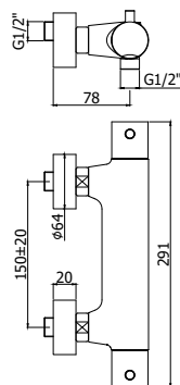
LIQ 168E-168EDCR Miscelatore termostatico doccia attacco 1/2" con/ senza set doccia, con limitatore di portata ECO-STOP Thermostatic shower mixer 1/2" connection with/ without shower kit, with flow reducer ECO-STOP
