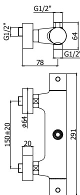
LIQ 169CR Miscelatore termostatico doccia attacco 1/2" x 1/2" con deviatore Thermostatic shower mixer 1/2" x 1/2" connection with diverter
