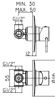
JK 010-011CR Miselatore incasso doccia / Piastra Ø116 e 110 mm Concealed shower mixer / Wall plate Ø116 and 110 mm
