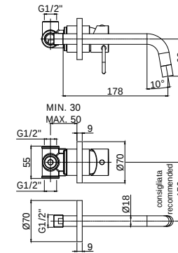
JK 006-007CR70 Miselatore incasso con bocca erogazione a muro 175 mm / 245 mm Concealed two-hole basin mixer with wall spout 175 mm / 245 mm
