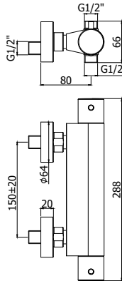
LIQ 469CR COULD TOUCH - ECOSTOP Miscelatore termostatico doccia attacco 1/2" x 1/2" con cartuccia deviatore Thermostatic shower mixer 1/2" x 1/2" connection with diverter cartridge
