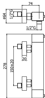
LEQ 268-268DCR Miscelatore termostatico doccia attacco 1/2" con/senza set doccia Thermostatic shower mixer 1/2" connection with/without shower set
